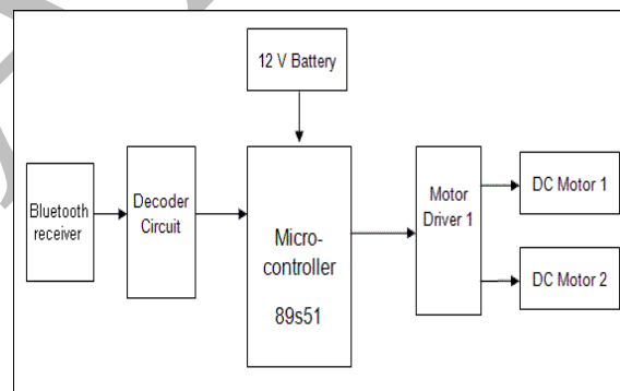
Figure 1.1: Block diagram of android smart phone controller Bluetoothrobot using 89s51 microcontroller
